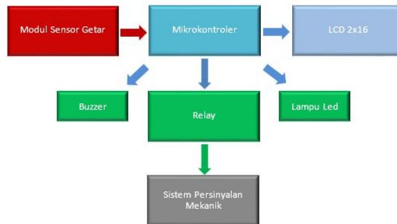
Figure 5: System Block Diagram
