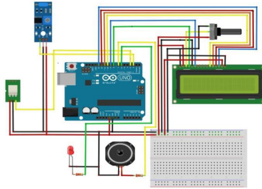
Figure 7: Detection System Design
