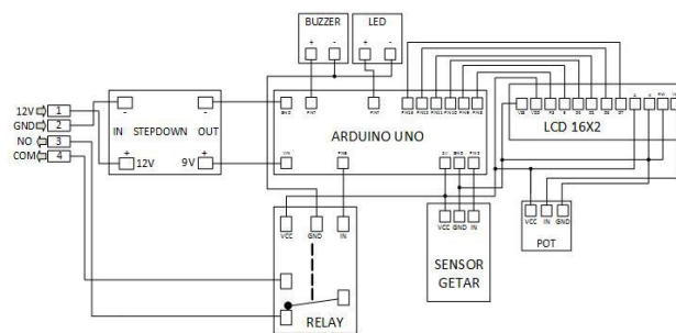
Figure 4: System Circuit Schema
