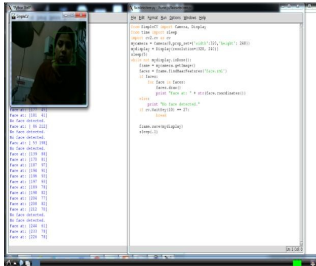
Figure 12. Face Detected and Tracking
