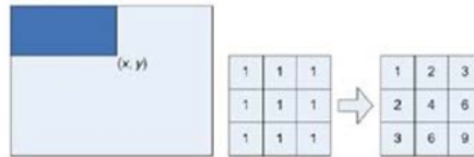
Figure 4. Integral Image generation. It shows a 3x3 image and its integral image representation
