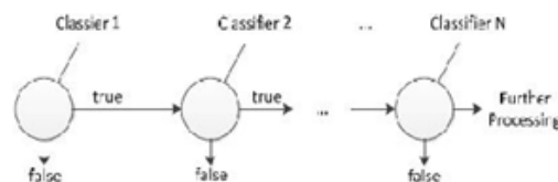
Figure 7. Cascaded of stages. Must pass all the stages to detect Face
