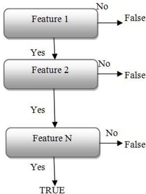
Figure 9. Decision tree based on Haar –like features (Cascade of classifier)
