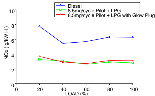
Figure 5: Variation of NOx with Load
