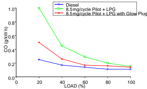
Figure 4: Variation of CO with Load
