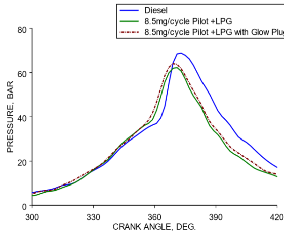
Figure 9: Variation of Pressure with Crank angle at Full Load
