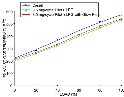
Figure 7: Variation of Exhaust gas temperature with Load
