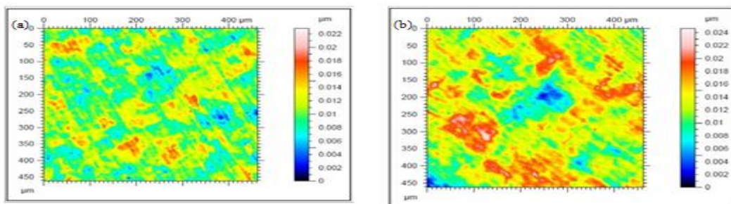
Fig 4.2 The surface roughness of workpiece (a) before nanoscale multi-tip tool cutting, and (b) after
