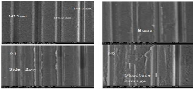
Fig 4.3 SEM images of Nano-grooves machined using different depth of cut. (a) 100 nm; (b) 200 nm; (c) 300 nm; (d) 400 nm. (Spindle speed = 12 rpm, feed rate = 9 μm/re).
