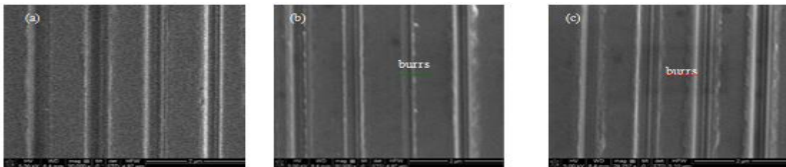
SEM images of nano-grooves machined under different spindle speeds. (a) 12 rpm; (b) 60 rpm (c) 120 rpm. (Depth of cut = 100 nm, feed rate = 9 μm/re).
