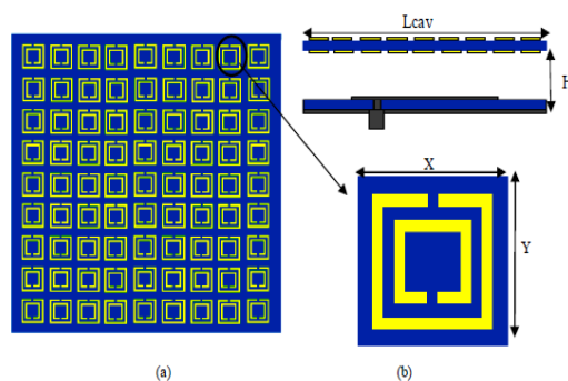
Fig. 1. Patch MMT double layer antenna. (a) top and front view of u
