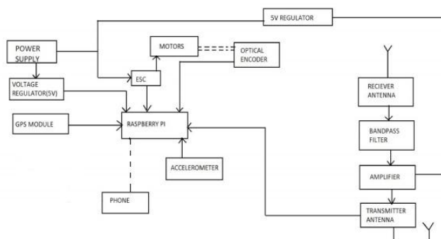
Fig.III.1(b) Block diagram of drone
