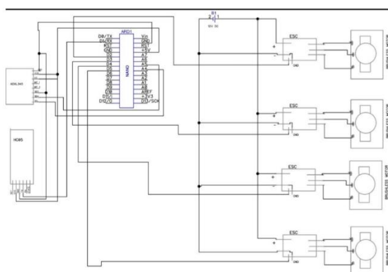
Fig. II.C Circuit Diagram
