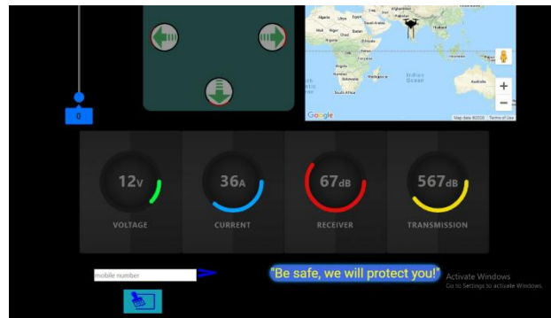
Fig. II.D Webpage
