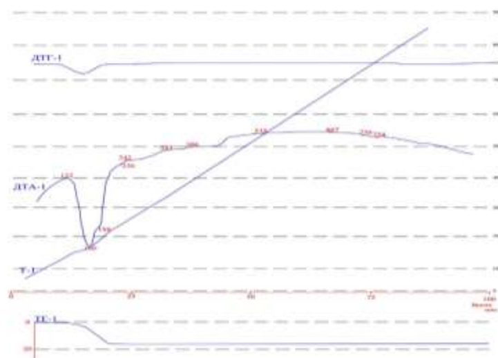
Figure 3a: DTA Sample Results Minaret Kalyan №.2B
