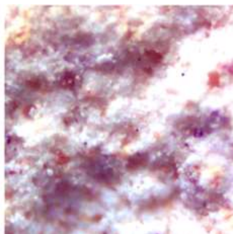
Figure 5b: The structure (x100) of the sample of the recommended modified masonry mortar (for restoration of the wall of the mausoleum of Ismail Samaniy)
