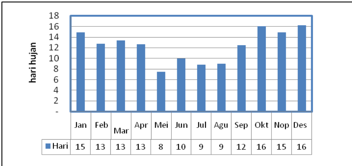
Figure 2: Day Average Monthly Rainfall Mahat Hulu Watershed (1995-2010)
