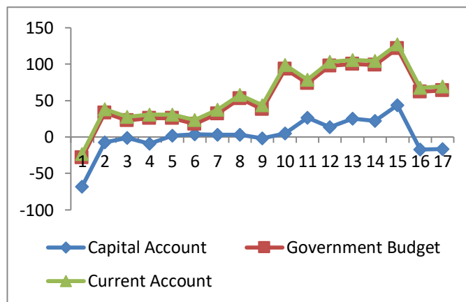
Figure 1: Performance Budget
