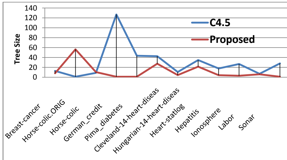
Figure 1: Trends in Tree Size for Proposed approach versus C4.5 on 12 datasets
