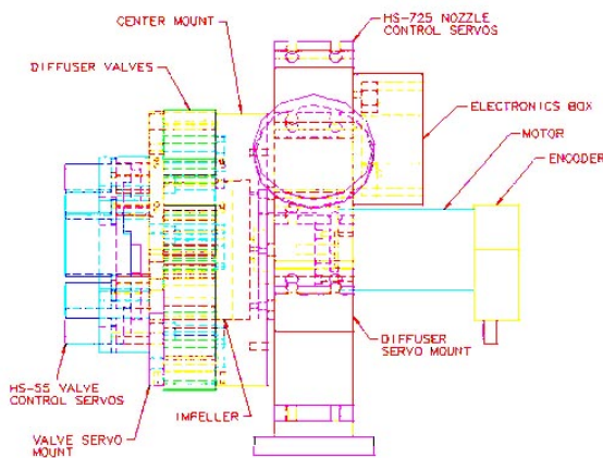
Figure 1: Main Center Assembly Figure 4: Diffuser Valve Assembly
