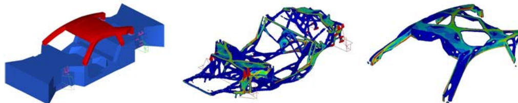
(a) domain, or design space (b) optimum chassis configuration (c) optimum roof configuration Figure 3:
