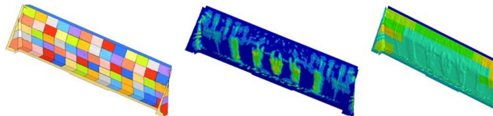
(a) Size optimization variables subdivision (b) Optimum configuration deformed shape (c) Damping material optimum thickness distribution
