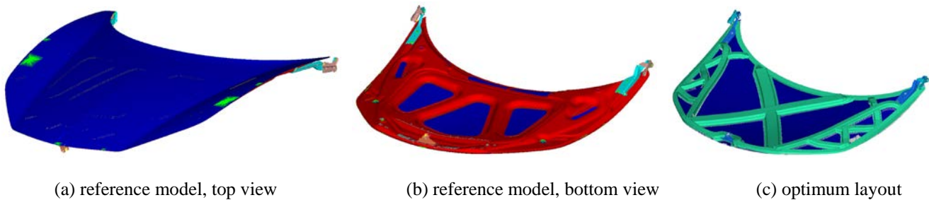
Figure 1: Ferrari F458 Italia front hood: reference model and new layout from the optimization results. The optimization was performed in three stages: topology, topometry, and size
